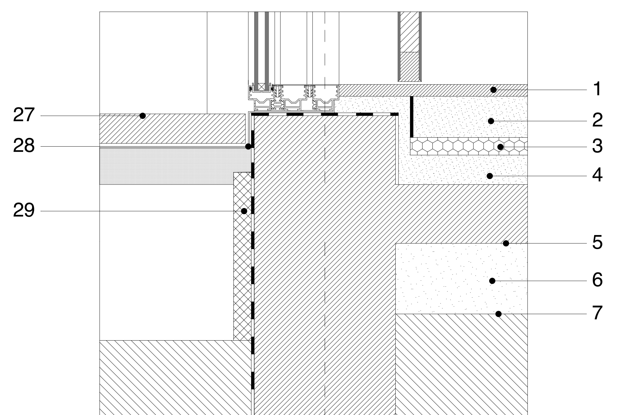
constructive section
