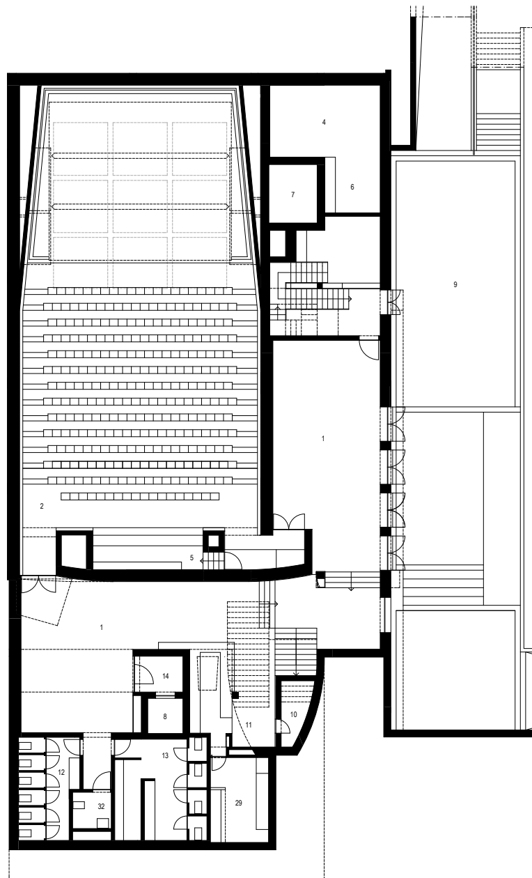
0 2 5 10m PLANTA CAVE
